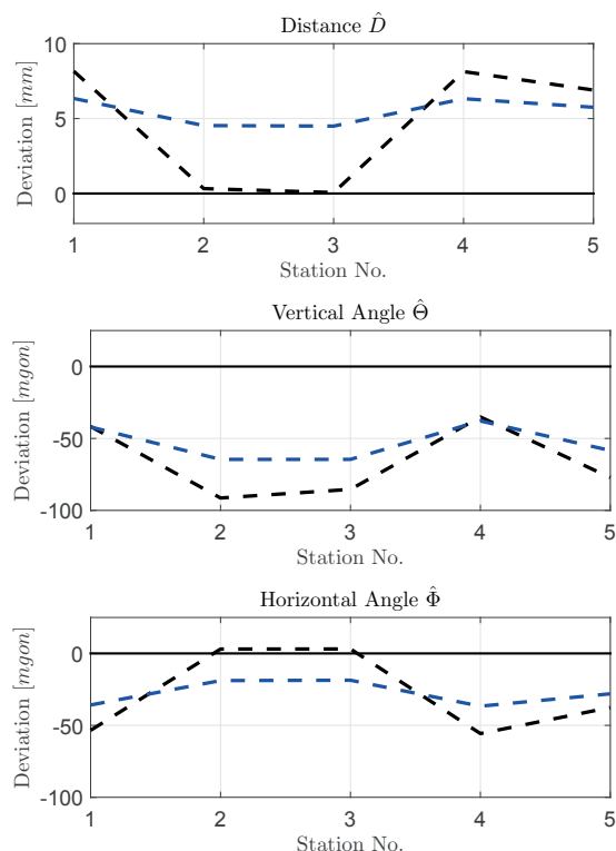
Fig. 10 | Simulated scanning of a deformed plane: biases of the parameter estimates depending on different laser scanner stations (black = original point cloud, blue = reduced point cloud) /Holst et al. 2014/
