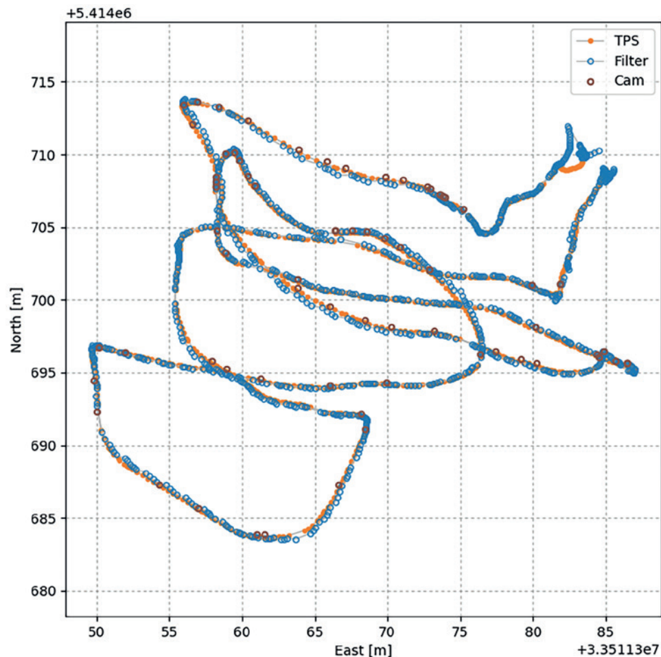
Fig. 10 | GNSS-IMU Filter results in blue, RTS-IMU (TPS) solution in orange and poses from bundle-block adjustment in brown
