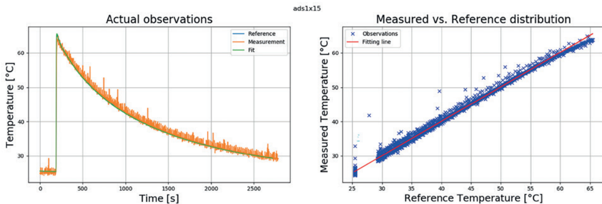
Fig. 6 | Temperature sensor calibration
