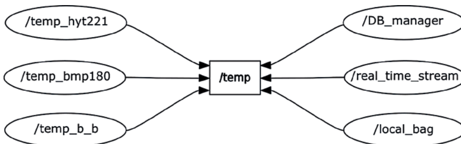
Fig. 2 | Example of simple RQT graph
