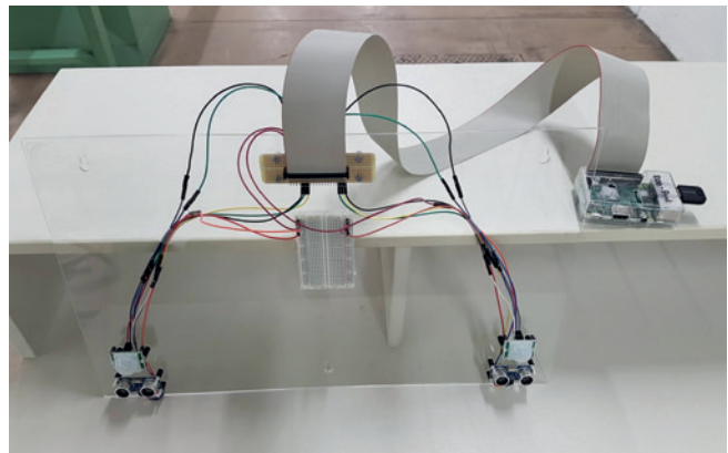
Fig. 7 | Mounting and control of motion detectors and ultrasonic distance sensors
