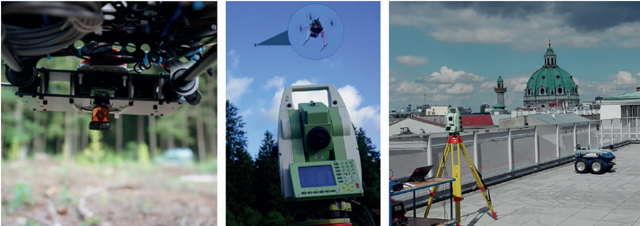
Fig. 9 | Prism mounted on UAV (left), RTS tracking UAV (center) and RTS tracking UGV (right)
