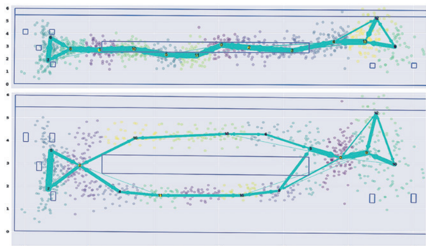
Fig. 8 | Raw smartphone positions (top) and refined positions with sensor infrastructure (bottom)
