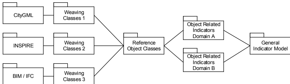
Fig. 5: Weaving Classes between different geospatial application models and the General Indicator Model
