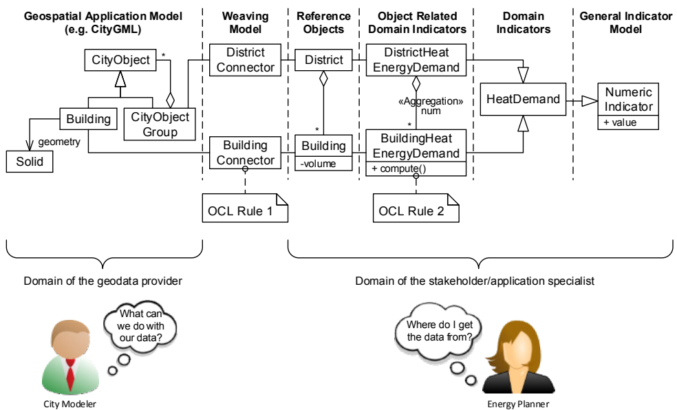
Fig. 4: Model Weaving Concept
